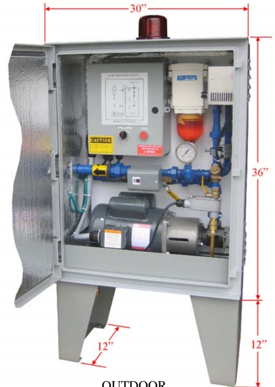
OUTDOOR ECLOSURE TYPE
